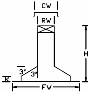
RAISED CANTED RAIL RCR
